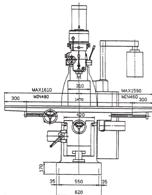
Machine Dimensions
